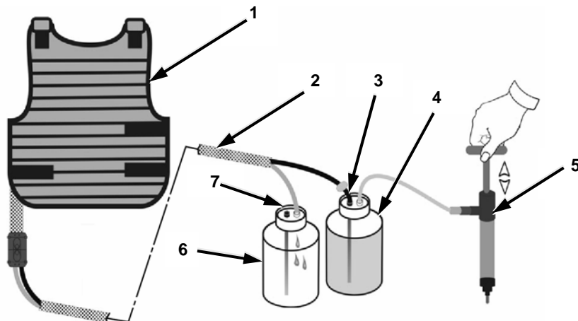
Figure 2-24. Charging MCG.
